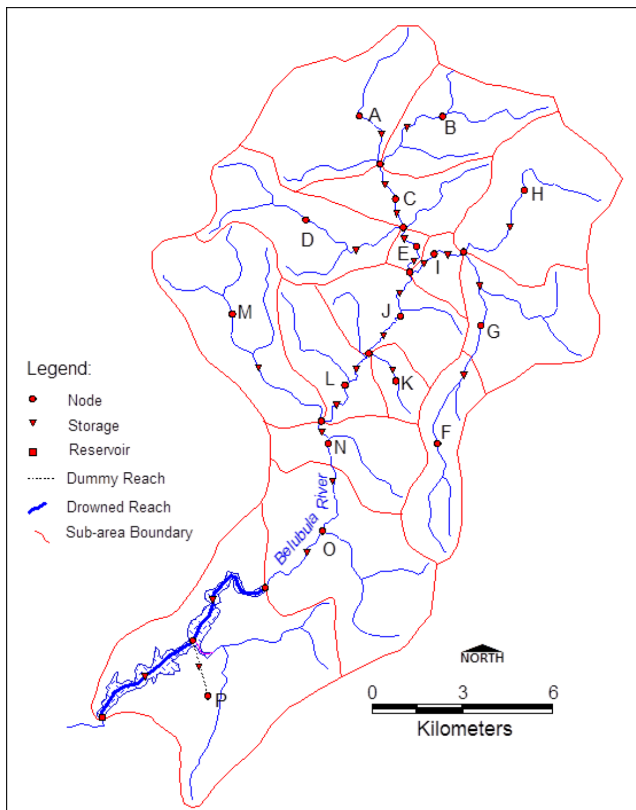
Figure C001 RORB Model Schematic
