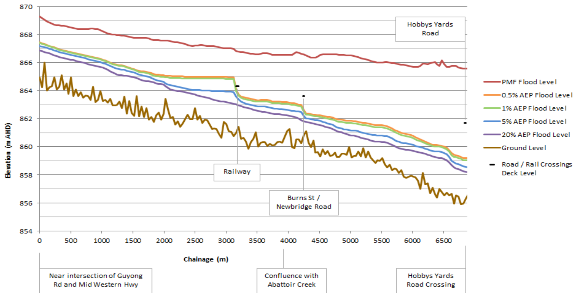
Figure 6-1 Peak Water Level Profiles – Belubula River
