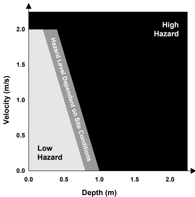
Figure 6-3 Hydraulic Hazard Category Diagram (reproduced from Figure L2 in NSW Floodplain Development Manual )
