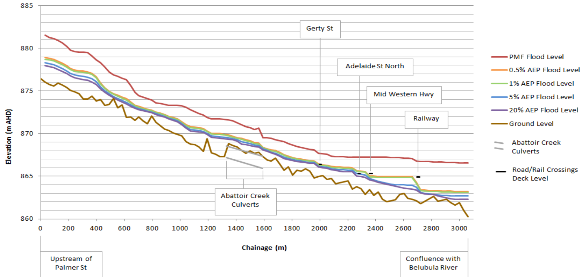
Figure 6-2 Peak Water Level Profiles – Abattoir Creek
