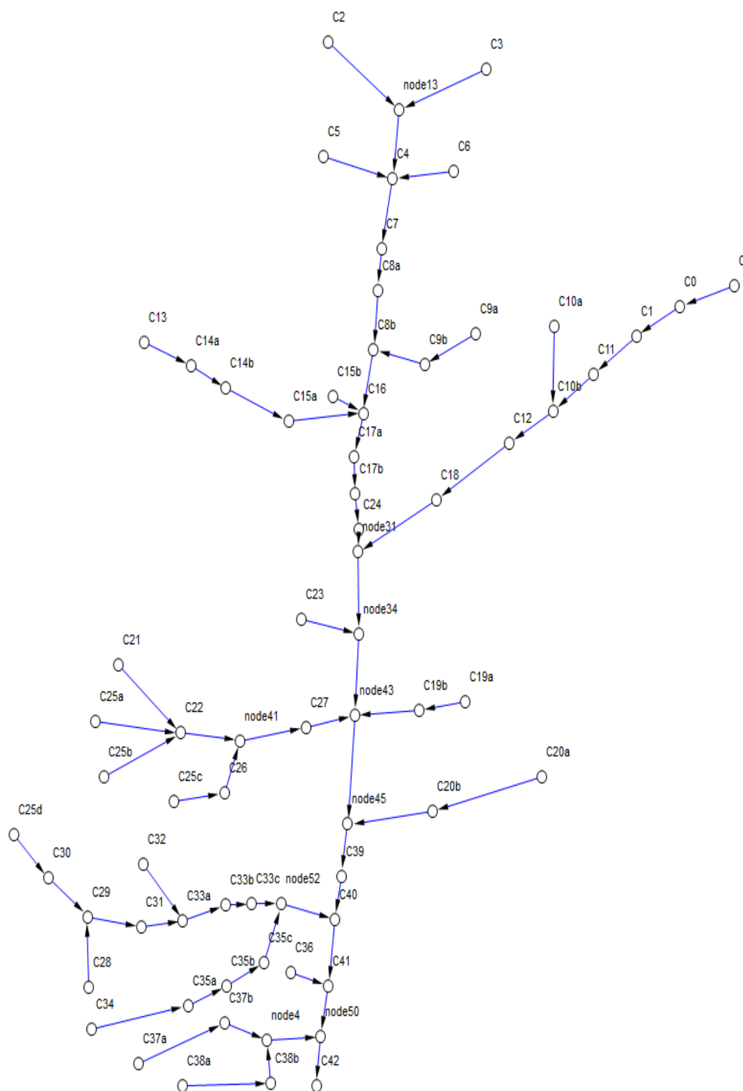
Figure C003 XP-RAFTS Model Schematic
